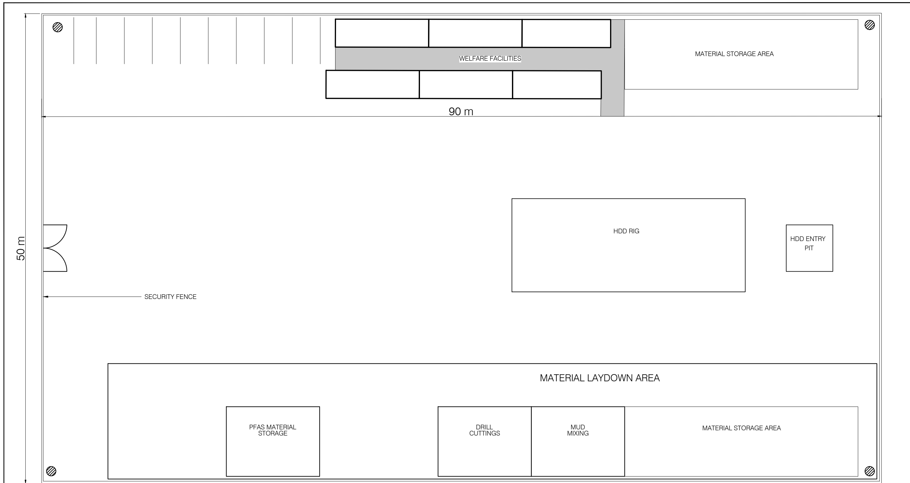
TYPICAL HDD COMPOUND/ LAYDOWN AREA SCALE 1:250
